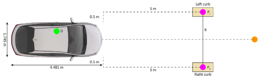
Fig. 1. Layout of the experiment. The green circle marked 'D' denotes the location of the driver, the orange circle marked 'S' denotes the location of the 'synchronizer' (i.e., the experimenter with the torch), and the magenta circles marked 'P L ' and 'P R ' denote the locations of the pedestrian on the left and right curbs, respectively. In the experiment, the curbs were rectangles (shown here in light brown), and the road crossing (marked 'R') was a line, all three drawn in chalk on the floor.
