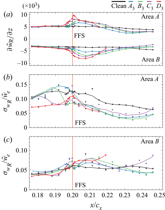
Figure 17. Streamwise evolution of averaged extracted values in areas A and B (defined in figures 15 and 16): (a) positive (area A) and negative (area B) averaged spanwise velocity gradients; (b) averaged velocity fluctuations in area A; (c) averaged velocity fluctuations in area B.
