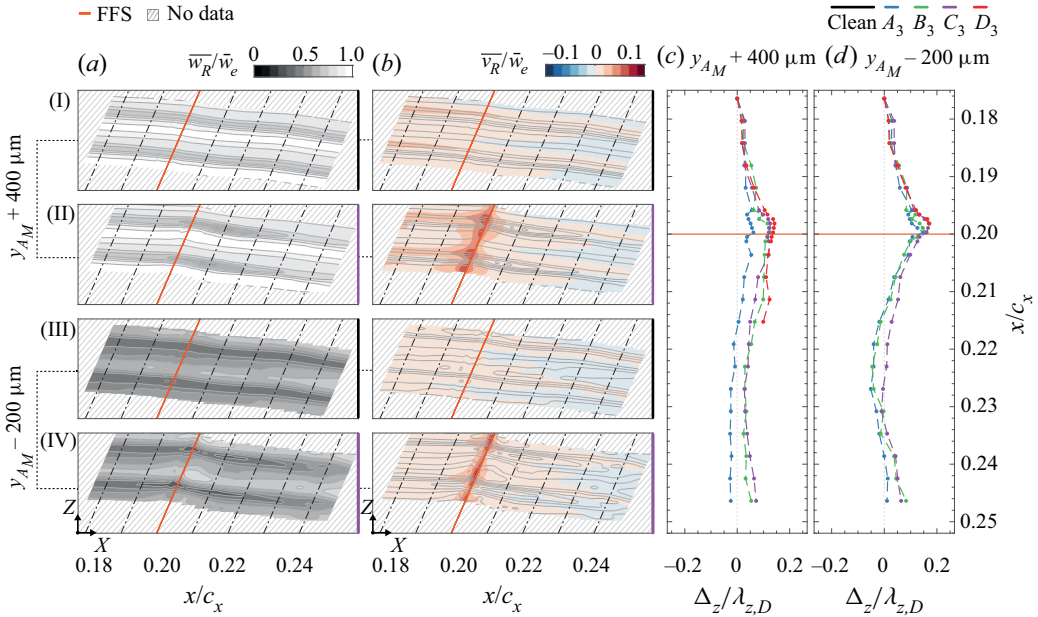
Figure 11. Wall-parallel contour maps of time-averaged spanwise and vertical velocity spatially filtered between \sum_m^5 m(0, n) . The contours in rows I and II are extracted at 400 \mu\text{m} above the height of the steady perturbation maxima ( y_{AM} ), while the contours in rows III and IV are extracted closer to the wall at 200 \mu\text{m} below y_{AM} : (I,III) clean case; (II,IV) C_3 case; and panels (c,d) the corresponding relative change of trajectory ( \Delta_z = dz_{SI} - dz_C ).
