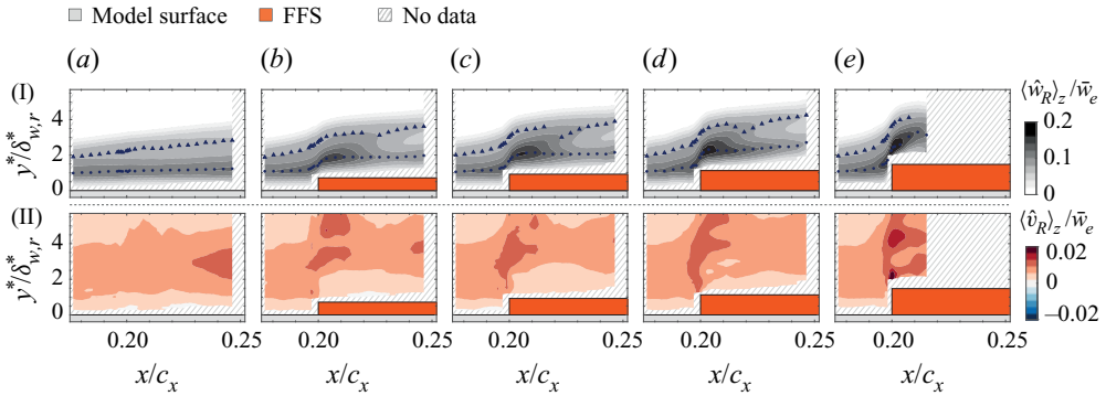
Figure 12. Contours of steady disturbances profiles (flow direction from left to right) \langle \hat{w}_R \rangle_z (I) and \langle \hat{v}_R \rangle_z (II) spatially filtered between \sum_n^5 m(0, n) . Location of lower (●) and upper lobe (▲): (a) clean; (b) A_3 ; (c) B_3 ; (d) C_3 ; (e) D_3 . (Here \delta_{w,r}^* = 514 \mu\text{m} ).
