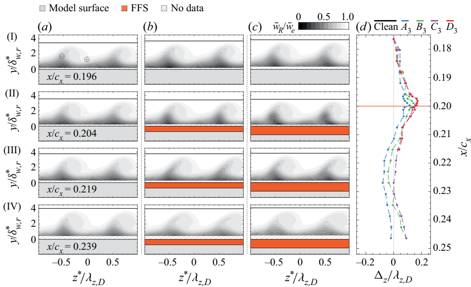
Figure 9. Contours of time-averaged spanwise velocity ( z^* positive direction outboard), spatially filtered between \sum_{n=1}^5 m(0, n) : (a) clean; (b) A_3 ; (c) C_3 ; (d) change in trajectory of the CF vortices due to the FFS. The solid black line denotes \delta_{99,w} (Here \delta_{w,r}^* = 514 \mu\text{m} and \lambda_{z,D} = 7.5 \mu\text{m} ).
