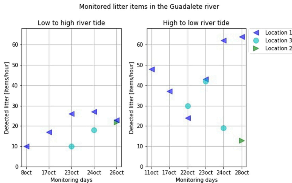
FIGURE 8 | Total monitored items during the field campaign using the wide scanning beam (47°), for the three different locations over the river's cross-section. Left: monitored items for river water level going from low to high (water flows from the sea inland). Right: monitored items for river water level going from high to low (water flows from inland towards sea).
