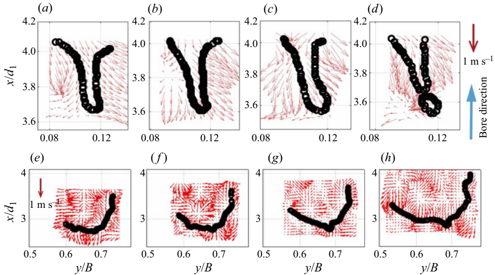
Figure 18. Flow fields obtained with the surface OF technique around a finger (a–d) and a crown (e–h). The time lapse between panels was t = 0.014 \text{ s} .
