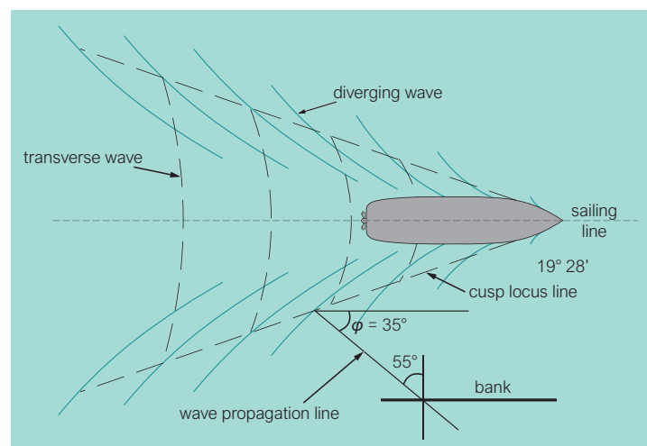
Figure 4.12: Locus of interference cusps (by TU Delft – Ports and Waterways is licenced under CC BY-NC-SA 4.0).
