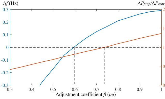
Fig. 11. Performance optimization of the proposed UFLS scheme by varying the adjustment coefficient.
