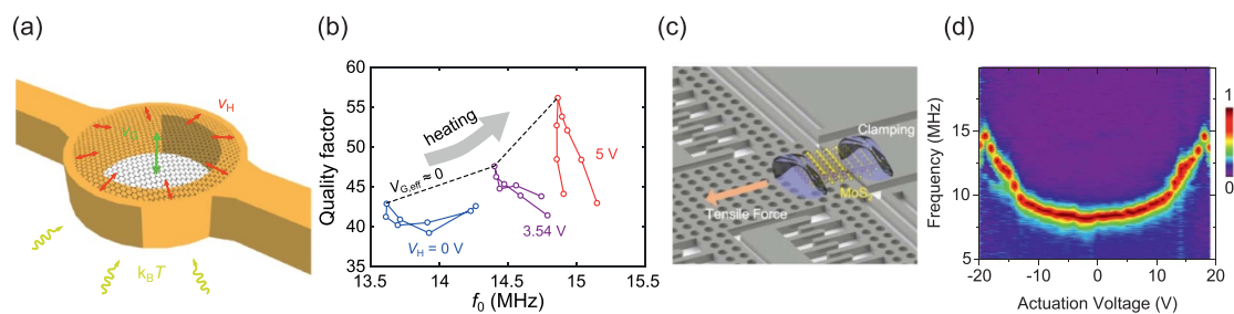
Figure 6. Engineering tension in 2D material resonators. (a) Schematic of a heater structure used to tension 2D material membranes. (b) Frequency versus quality factor plot at different heater voltages. (c) Schematic of a comb-drive actuator to tension 2D material membranes. (d) Resonance frequency tuning of a 3-layer MoS 2 resonator using a comb drive actuator. Figures (a) and (b) are reprinted from [93] licensed under CC-BY-NC-ND. Figures (c) and (d) are reprinted with permission from [117], copyright (2020) Wiley-VCH GmbH.
