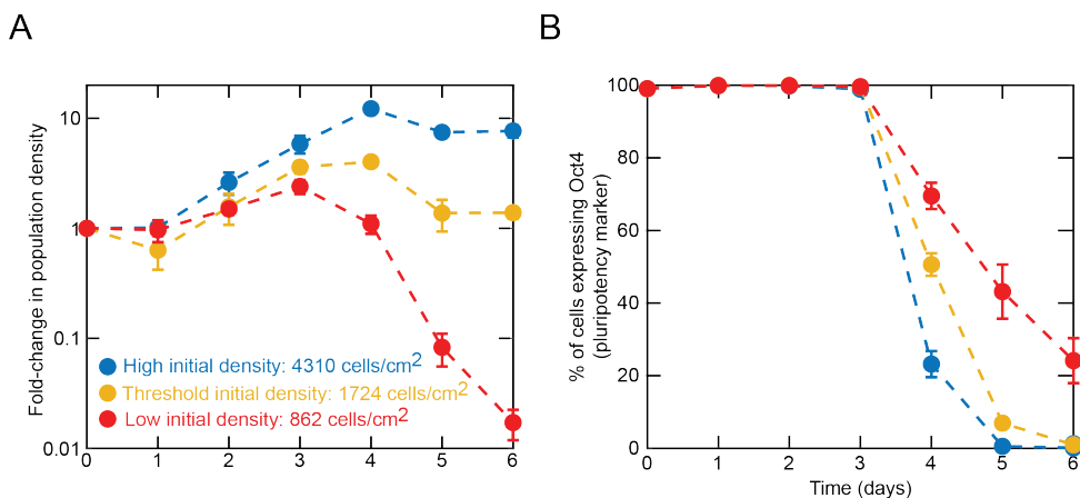
Figure 2.8: Initial population density determines the rate of loss of the pluripotency marker Oct4 during differentiation. Data shown for Oct4 -GFP cell line (a kind gift from Austin Smith, also see [116, 174]). This cell line has the Oct4 promoter controlling GFP expression. Different colors represent different initial population densities as indicated in the legend (4310, 1724, and 862 cells / cm 2 ). For each differentiation, we took the pluripotent cell line (previously cultured in 2i+LIF) and then started differentiation with the indicated initial population densities, adding Retinoic Acid (RA) into N2B27 medium after 2 days (i.e., on day 2). As seen here, the Oct4 degradation (as measured by the % of cells expressing GFP) during differentiation, and therefore the loss of pluripotency depends on the initial population density. n = 3 ; error bars are s.e.m. On day 4 of differentiation high-density populations (shown in blue) have ~20% Oct4 -GFP positive cells whereas low-density populations (shown in red) still have ~70% Oct4 -GFP positive cells. Intriguingly, on day 5 nearly-extinct low-density populations still comprise ~50% Oct4 -GFP positive cells, whereas high-density populations (at carrying capacity) have virtually none. These results complement our findings on differentiation efficiencies (Supp. Fig. 2.11).
