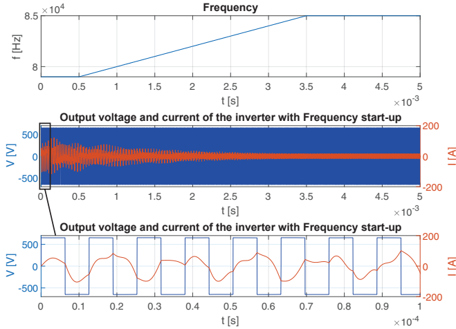
Fig. 10. The output voltage and current of the inverter with frequency control for LCC-LCC compensation, duty cycle = 0.5.
