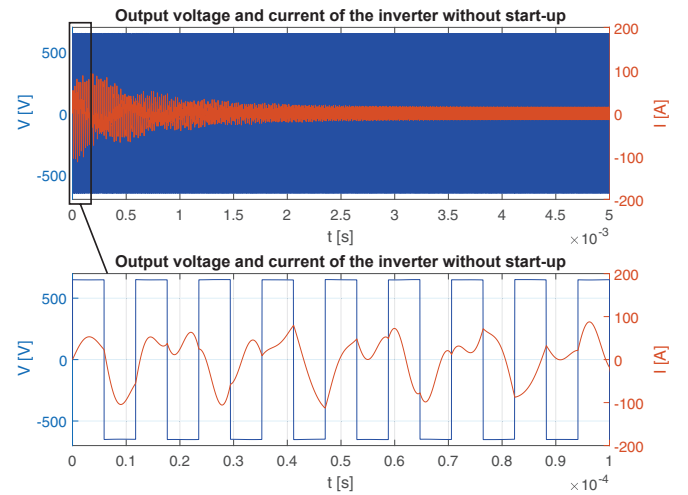
Fig. 8. The output voltage and current of the inverter without soft start-up for LCC-LCC compensation, frequency = 85 kHz.
