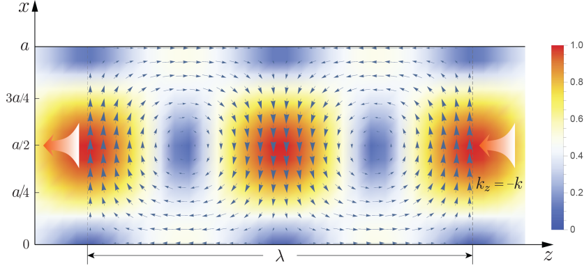
Figure 1.2: The spatial distribution of magnetic field \mathbf{H} for the TE 10 mode which has lowest dispersion band in the rectangular waveguide. The arrows shows the direction of \mathbf{H} field and the color shading indicates its relative magnitude.
