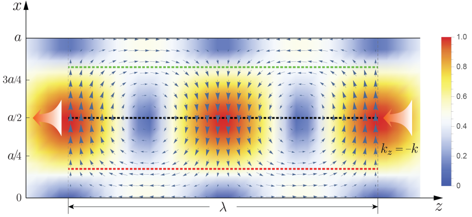
Figure 4.2: Snapshot of the spatial distribution of the AC magnetic field of the lowest TE_{10} mode in a rectangular waveguide propagating along the -z -direction. The arrows indicate the direction and modulus of the field. The latter is also indicated by the color shading, from zero (dark blue) to maximum value (dark red). The vector field of modes along the z -direction (not shown) is reversed. The green and red (black) dotted lines indicate the locations at which the magnon-photon coupling is chiral (non-chiral) for magnon frequency tuned to \omega_l = \sqrt{5}c\pi/a . On the red (green) line, the magnon mode only couples to photons with positive (negative) linear momentum.
