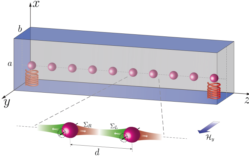
Figure 4.1: Chain of magnetic spheres with period d in a microwave waveguide. The chain and waveguide are parallel to the \hat{z} axis and magnetizations are oriented along \hat{y} axis by a magnetic field H_y . Every magnet interacts with all other magnets to the right ( \Sigma_R ) and to the left ( \Sigma_L ). Small coils attached to magnet can excite and detect the local magnon accumulation.
