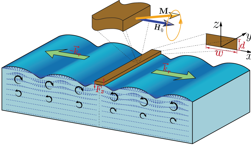
Figure 2.1: Surface-phonon pumping by one magnetic nanowire (brown) on top of the acoustic insulator (blue). A static magnetic field H_0 applied in the \bar{x} direction saturates the magnetization. The pumped Rayleigh SAWs by the nanowire FMR propagate and rotate in opposite directions at the two sides of the nanowire as indicated by the green and black arrows, respectively.
