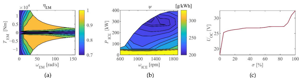
Figure 7. (a) Efficiency map of an electric motor; (b) specific fuel consumption of an internal consumption engine; and (c) lithium-ion battery module open circuit voltage as a function of state-of-charge.
