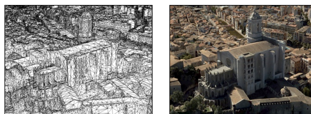
Figure 5 Hyperrealistic textured triangulation from the oblique images
