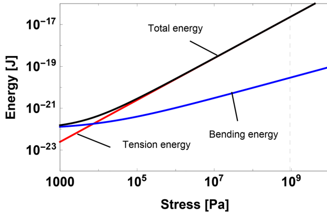
FIG. 1. Energy diagram for the (0,1) mode of a round-shaped nanomembrane resonator with dimensions D = 1480\ \mu\text{m} , thickness h = 100\ \text{nm} showing the contribution of the tensile, the bending energy, and the total energies by varying internal stress \sigma .
