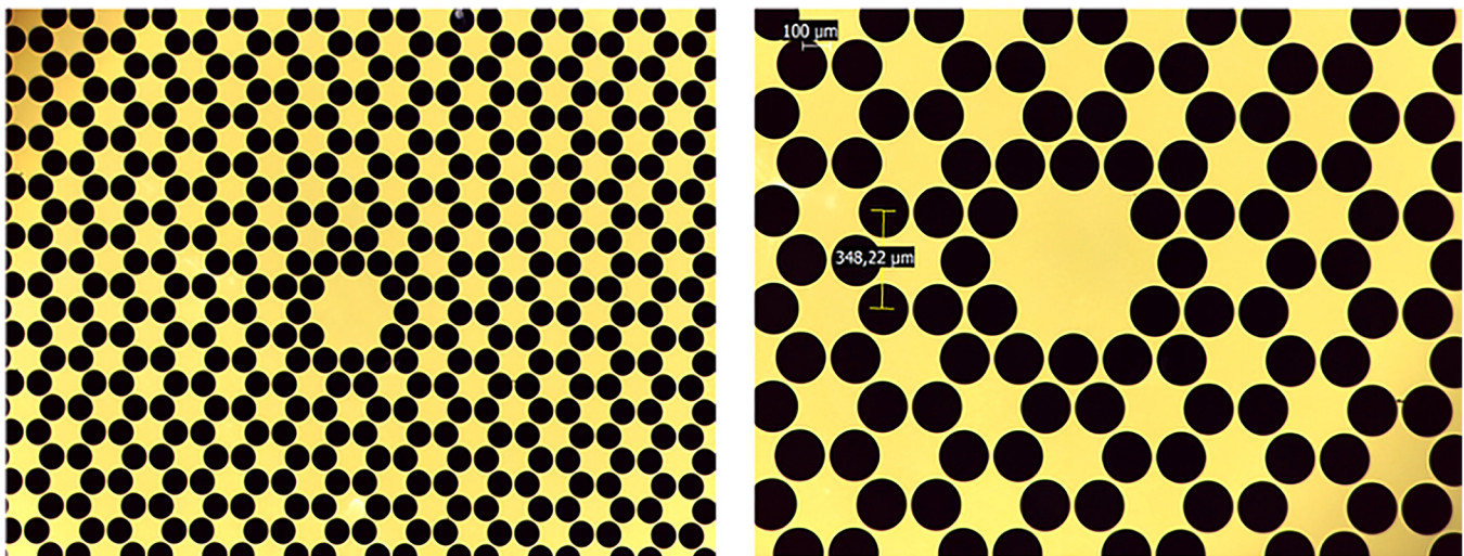
FIG. 8. Phononic bandgap lattice ( a = 346\text{ }\mu\text{m} ) (left) with a detailed view of the central resonating part (right) with the hexagonal-shaped defect region in the center of the lattice.
