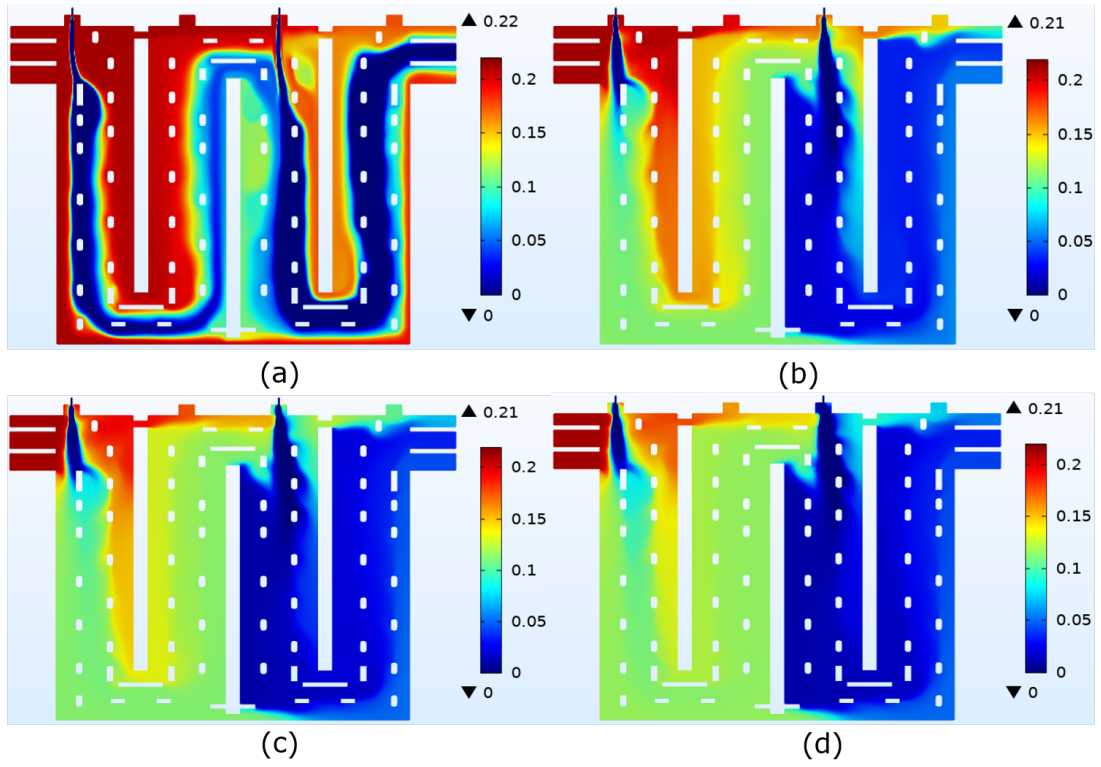
Figure 13. Mass fraction of O_2 at XY plane ( Z=0.27 m) for (a) \delta_{id} = 0 , (b) \delta_{id} = 0.1 , (c) \delta_{id} = 0.3 and, (d) \delta_{id} = 0.5 . The diffusion improves as the tuning parameter increases from 0 to 0.5. This leads to wider reaction zones with increase in the tuning parameter. Therefore, the lower mass fraction of O_2 at the outlet is not restricted to a narrow stream for higher tuning parameters as observed from measurements.
