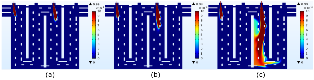
Figure 15. The \text{CH}_4 mass fraction distribution at the symmetry plane for varying fuel inlet mass flow rate of (a) 0.002 kg/s (b) 0.003 kg/s and (c) 0.0037 kg/s with 9 mm fuel pipe diameter. The higher mass flow rate results in the higher momentum of the jet as well as higher amount of \text{CH}_4 mass fraction. Therefore, the region of unreacted \text{CH}_4 is higher with increased mass flow rate.
