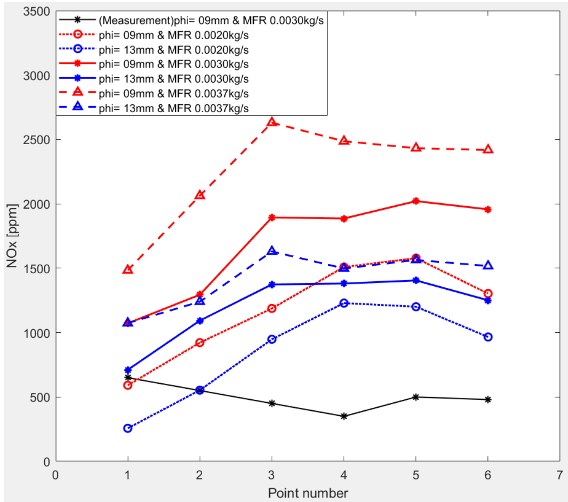
Figure 24. NOx fraction at six measured point locations for varying fuel pipe diameters and fuel injection velocities. Red and blue colors denote the results of 9 mm and 13 mm diameter fuel pipes, respectively. Black color denotes the measured values for 9 mm diameter and 0.003 kg/s. Symbols '★', 'o' and 'Δ' represent values for mass flow rate of 0.003 kg/s, 0.002 kg/s and 0.0037 kg/s, respectively. NOx calculated from the model are over predicted as compared to measured values. With increased fuel pipe diameter, NOx decreases for a certain mass flow rate of fuel. While, NOx increases with increase mass flow rate of fuel for a certain fuel pipe diameter.
