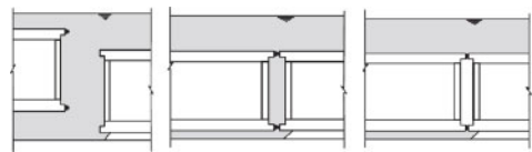
Figure 1. Construction procedure of immersion joint.
