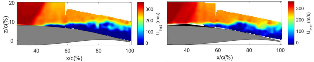
Fig. 6 Example of a PIV image of the OAT15A at Ma=0.7 , \alpha=3.5^\circ with bumps ( right ) and without ( left ).
