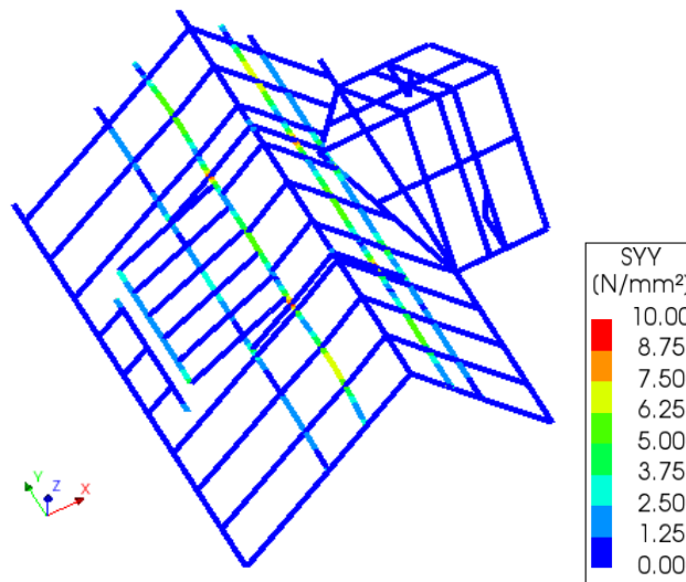
Figure 53. Peak of global Y stress of roof beams.
