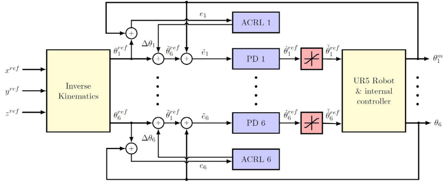
Fig. 3. RL reference compensation framework for the joint space trajectory. In this case, the method is applied to a 6-DoF robot, e.g., the UR5. A RL-based compensator is learned for each joint separately using the actor-critic framework. Here the correction is added to the reference signal.
