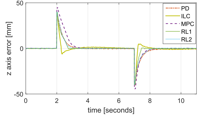
Fig. 6. The tracking performance of the proposed RL compensation methods compared to the benchmark controllers for the square reference.
