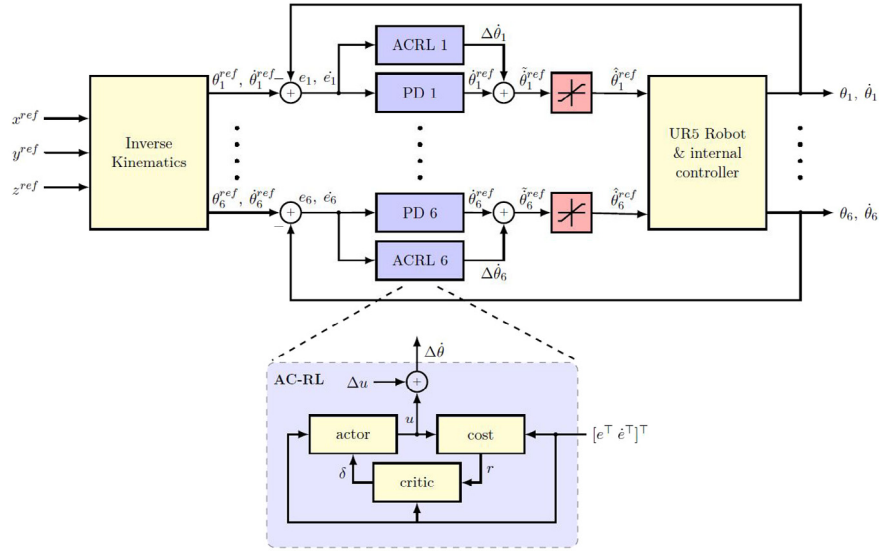
Fig. 2. RL control input compensation framework for a 6-DoF robot, e.g., the UR5. A RL-based compensator is learned for each joint separately using the actor-critic framework. Here the correction is added to the control action.
