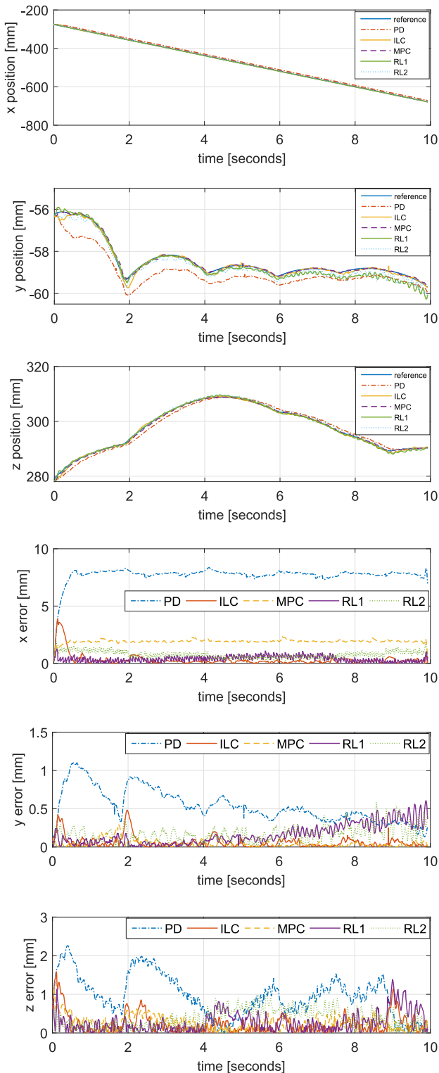
Fig. 11. Reference tracking result of the 3D printing reference task using RL controllers. Top to bottom: the reference and measured x , y and z trajectory of the end-effector, absolute tracking error on x , y and z axes.
