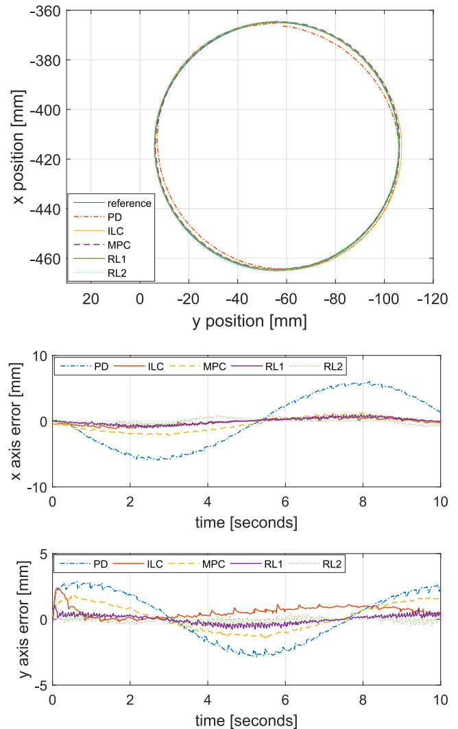
Fig. 8. Top to bottom: the x - y trajectory of the RL methods compared to other control methods for the circular reference, x axis error, y axis error.
