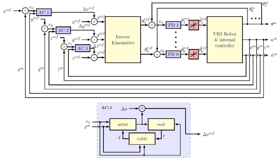
Fig. 4. RL reference compensation framework for the Cartesian space trajectory. A RL-based compensator is learned for each Cartesian direction separately using the actor-critic framework. Here the correction is added to the reference signal.
