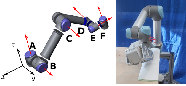
Fig. 5. The UR5 Robot. Left: The joint's axis positioning and the reference frame used in this paper. The joints in alphabetical order (A to F): base, elbow, shoulder, wrist 1, wrist 2, and wrist 3. Picture is courtesy of Universal Robots. Right: the 3D printing system with the robot moving on top of the surface of a curved object.
