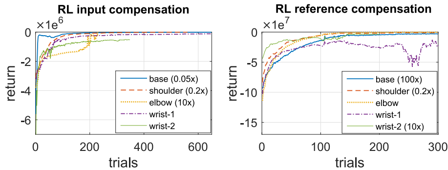
Fig. 10. The discounted sum of rewards (return) of each learning agent for the 3D printing reference. Note that appropriate scaling to the discounted return curves is applied for readability. Furthermore, the number of trials per agent can be different, as shown with different number of trials per agent.
