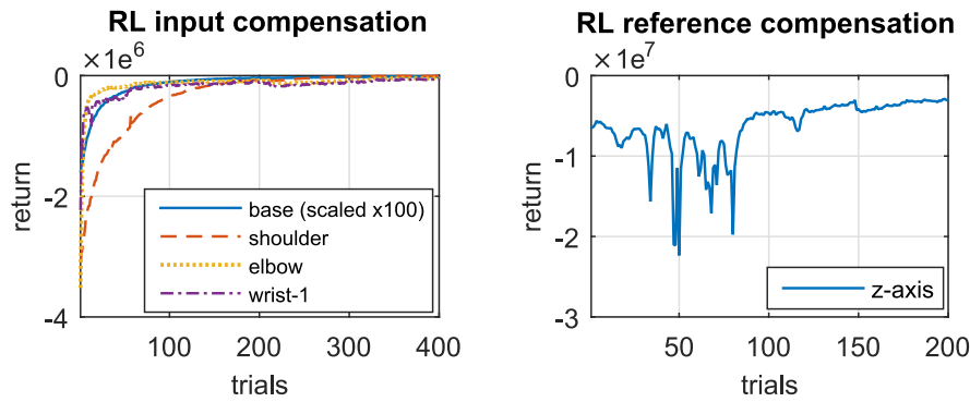
Fig. 7. The sum of rewards (return) of all the learning agents for the square reference. Left: RL input compensation, right: RL reference compensation. Note that appropriate scaling to the discounted return curves is applied for readability.
