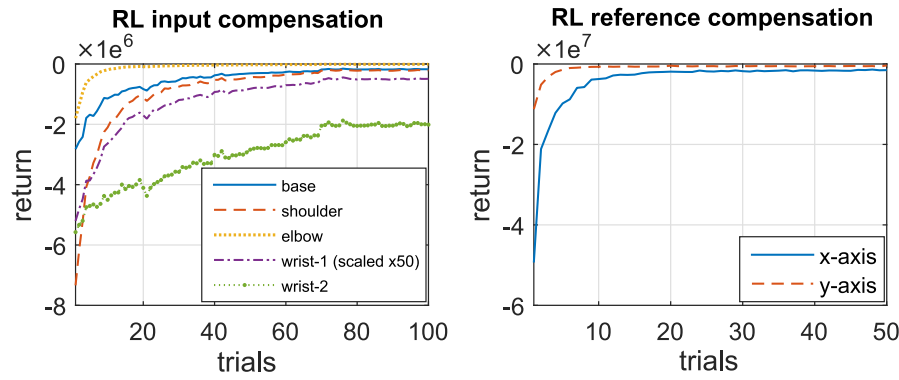
Fig. 9. The sum of rewards (return) of all the learning agents for the circular reference. Left: RL-input compensation, right: RL reference compensation. Note that appropriate scaling to the discounted return curves is applied for readability.
