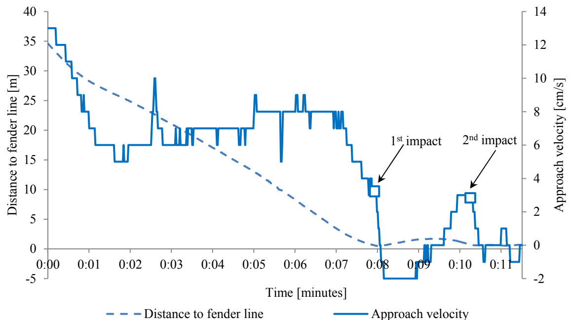
Figure 4: Approach velocity at moment of impact recorded with SmartDock® portable workstation of Post-Panamax container vessel
